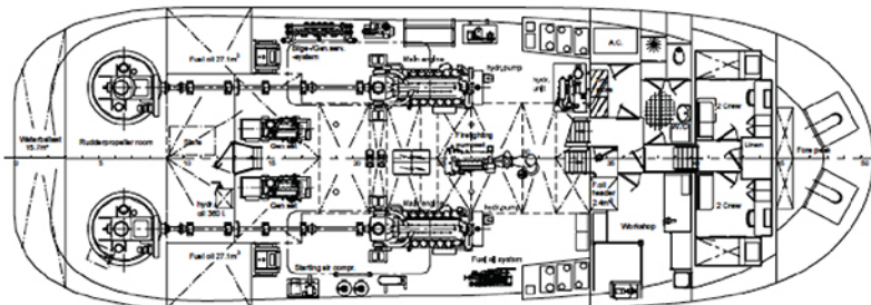
Below Maindeck
